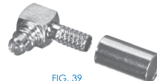
FIG. 39 RP-9010-1B (shown at 200% size)
